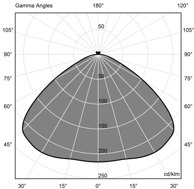
Light Distribution POLAR DIAGRAM
