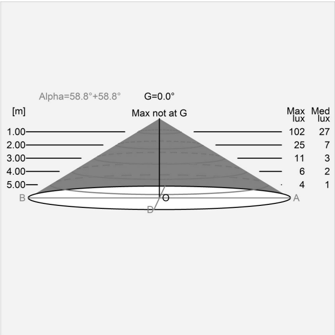
Light Distribution CARTESIAN
